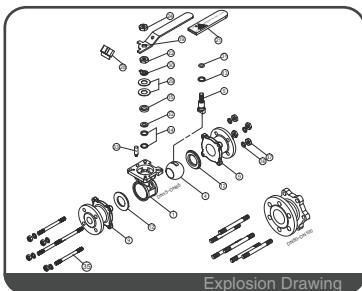
Exploded Drawing
